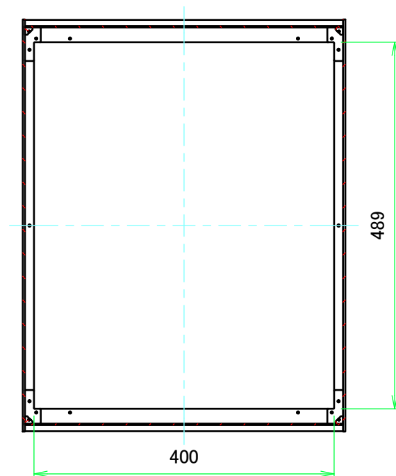
B-B (1:7)
