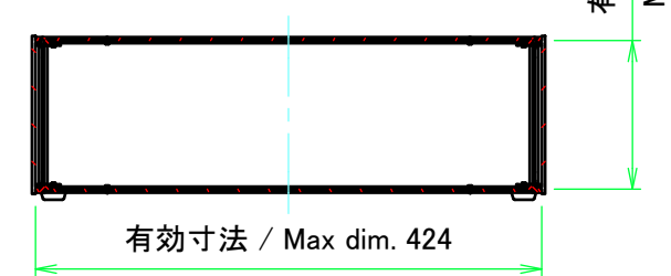
C-C (1:7)
