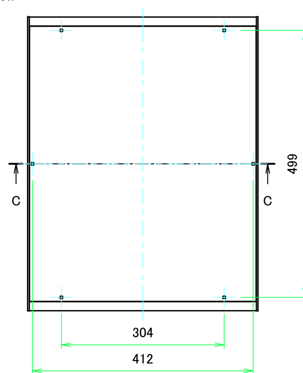
E view
