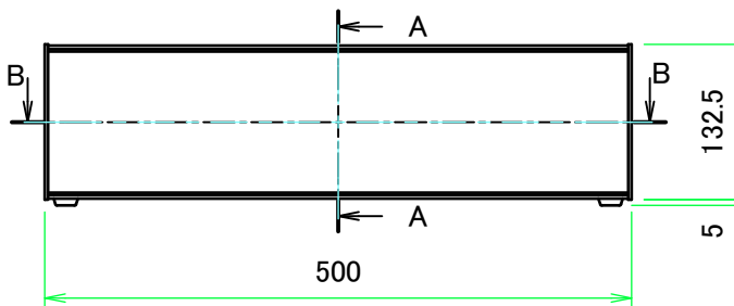
A view
