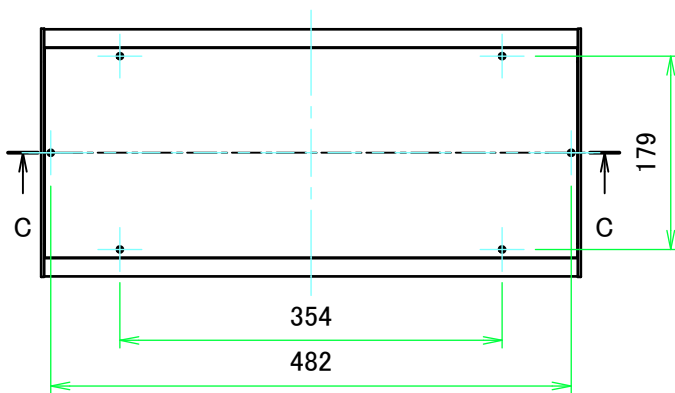
E view
