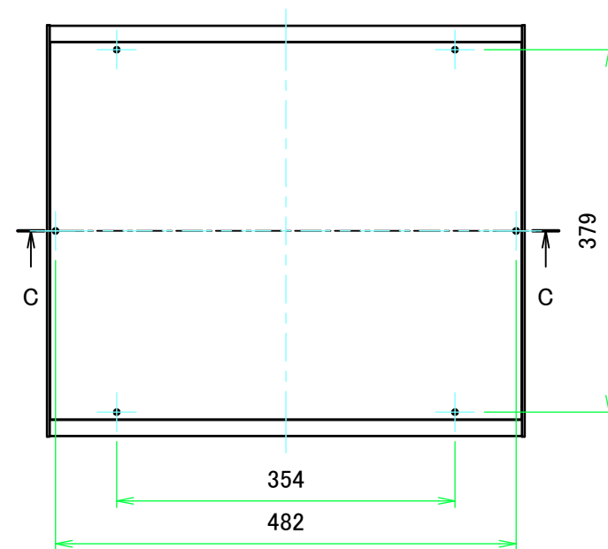
E view
