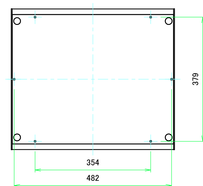
F view
