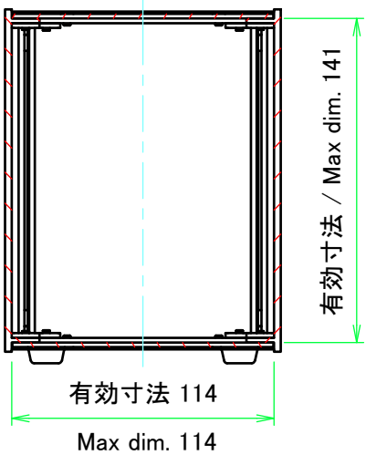
C-C (1:3)
