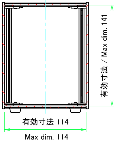
C-C (1:3)
