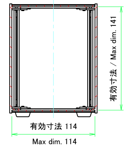
C-C (1:3)
