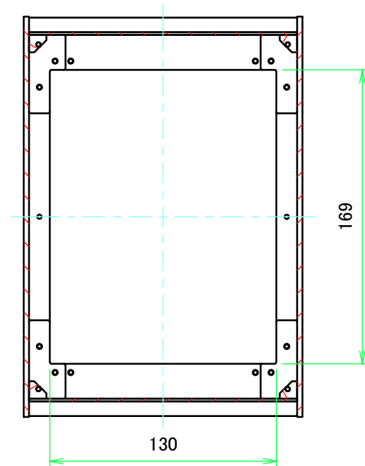
B-B (1:3)
