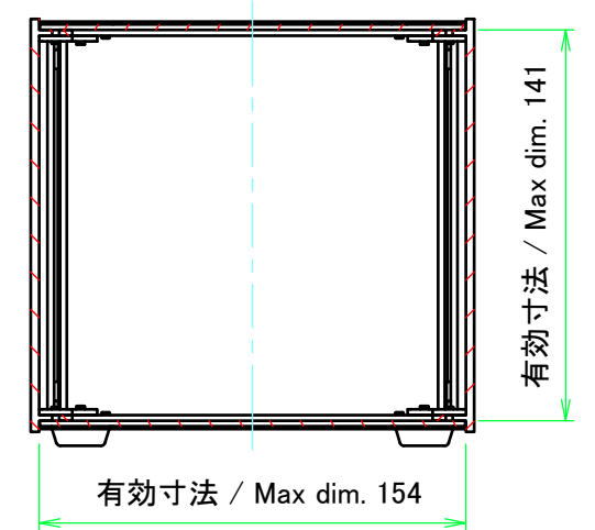
C-C (1:3)
