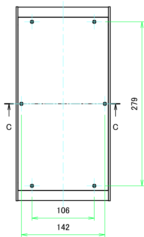
E view
