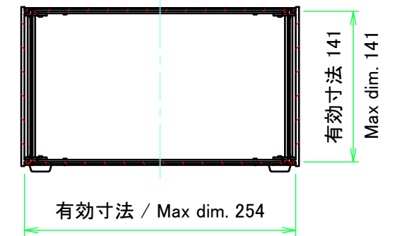
C-C (1:5)
