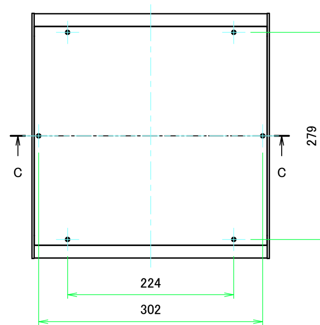
A view
