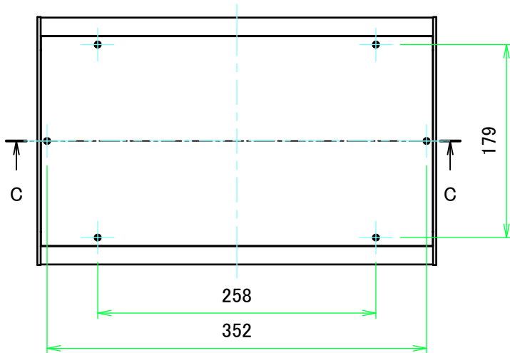
E view
