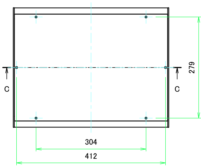
A view
