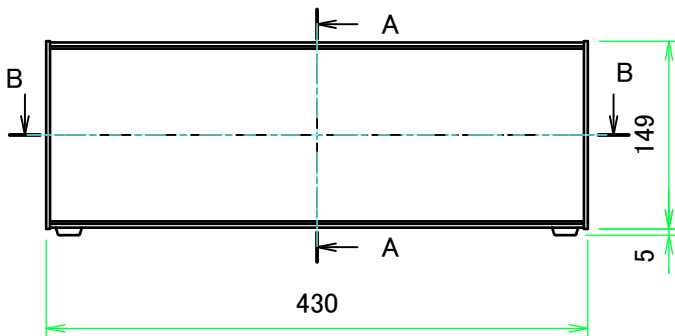
F view
