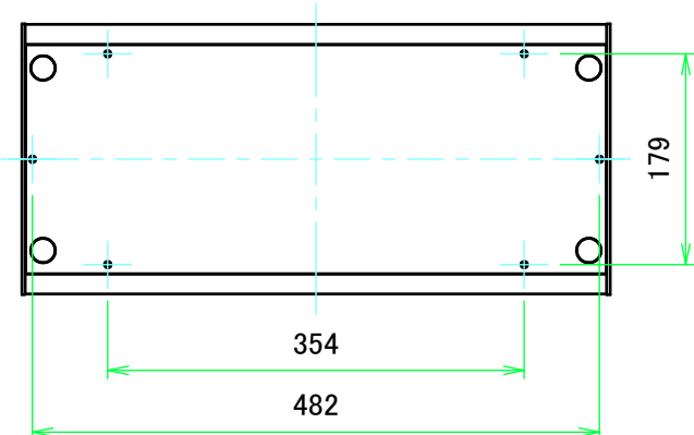
F view
