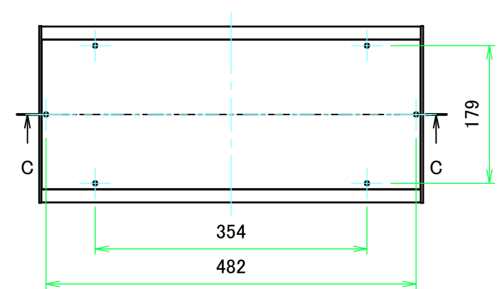
E view
