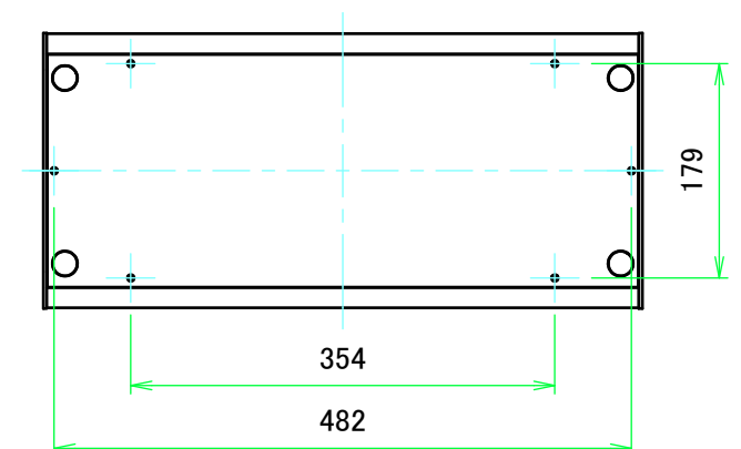
F view
