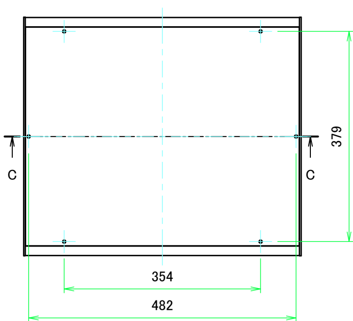
E view
