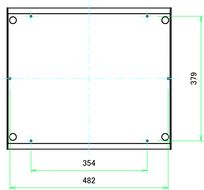
F view
