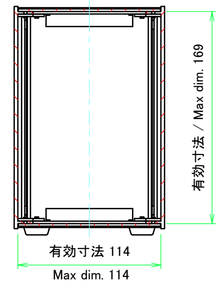
C-C (1:3)
