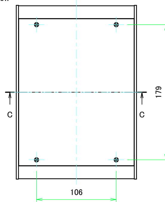
E view
