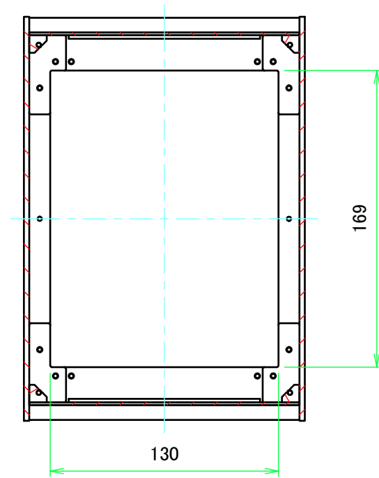
B-B (1:3)
