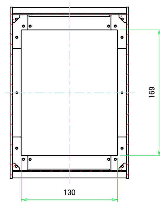
B-B (1:3)
