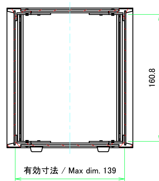
C view
