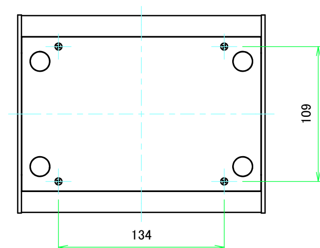
F view
