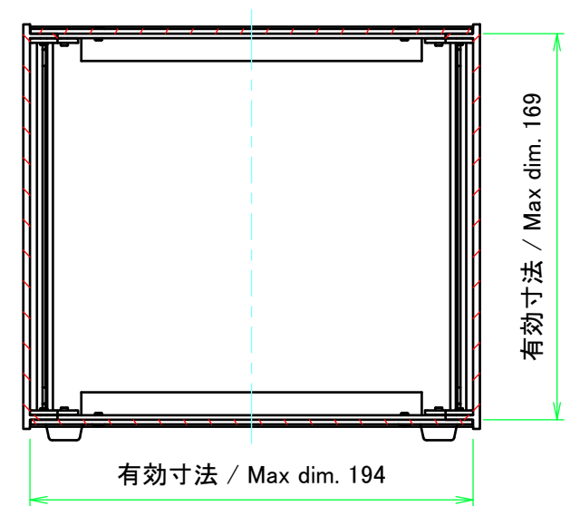
C-C (1:3)
