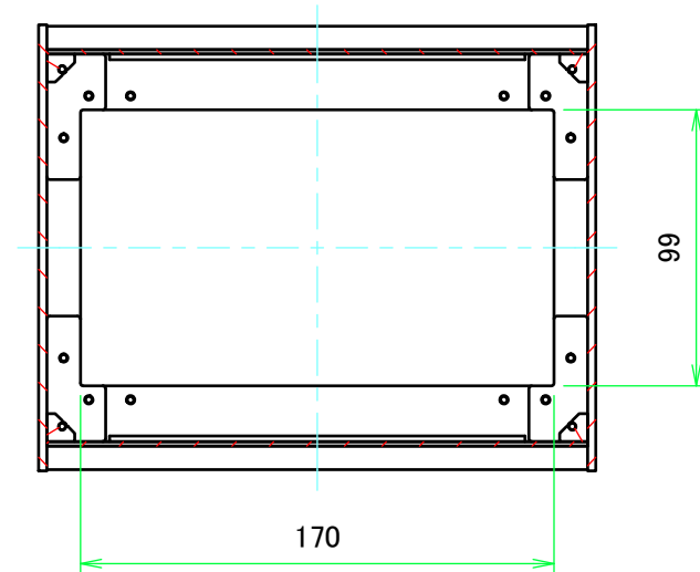
B-B (1:3)
