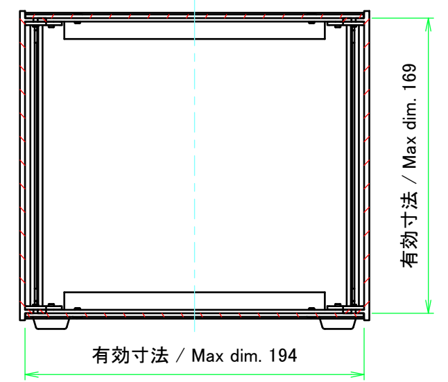
C-C (1:3)
