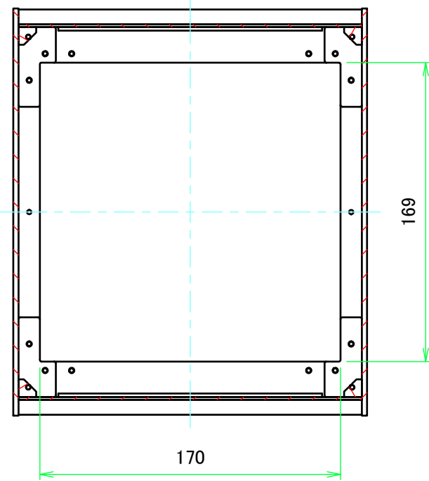
B-B (1:3)
