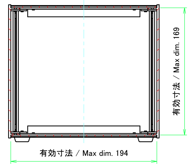
C-C (1:3)
