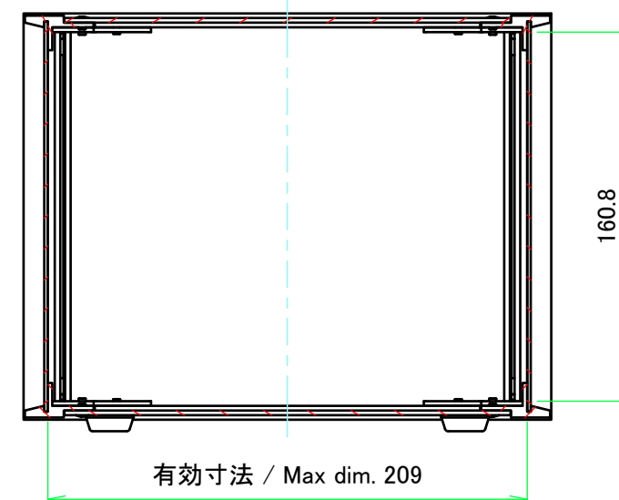
C view
