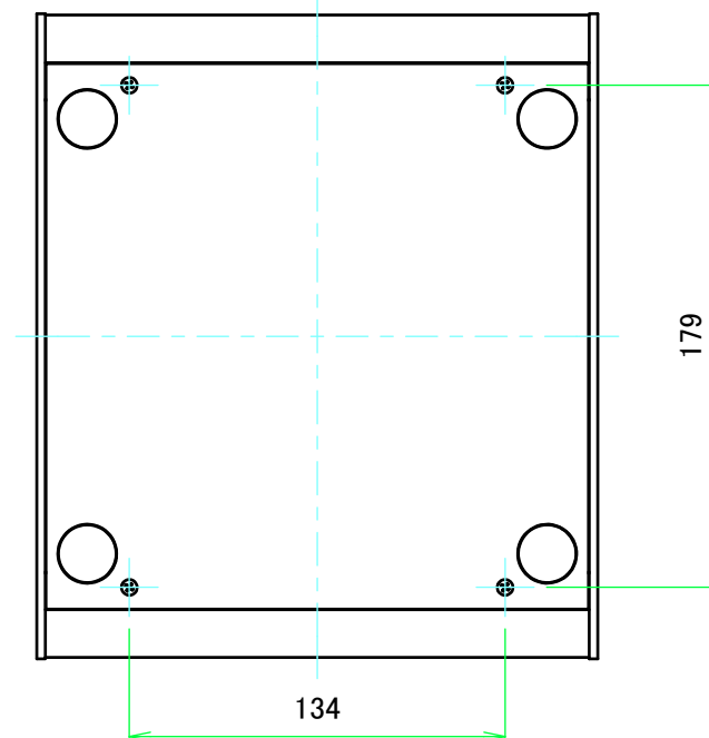
F view
