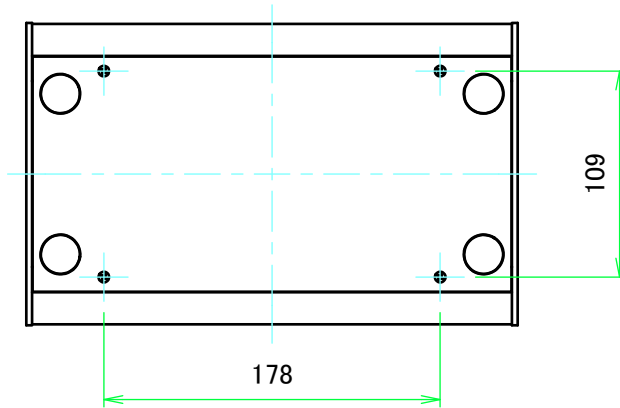
F view
