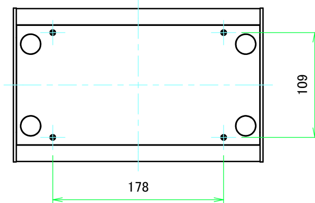
F view
