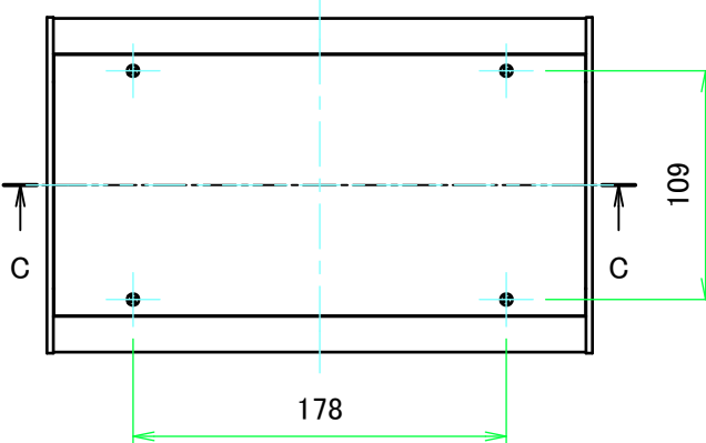
E view
