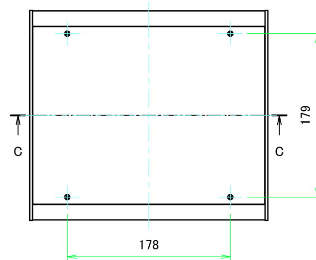
E view
