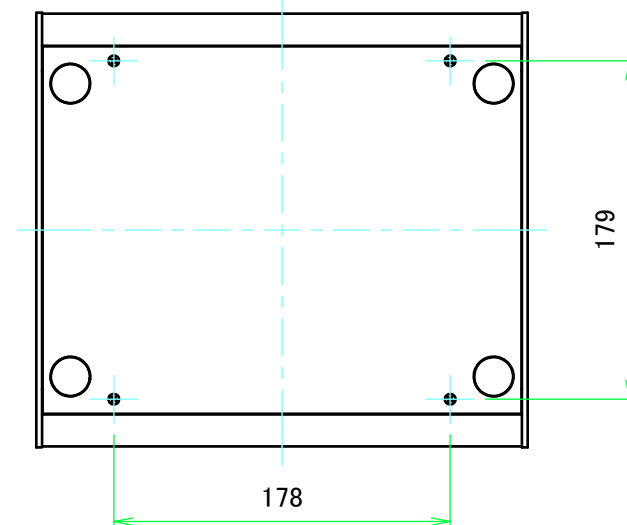
F view
