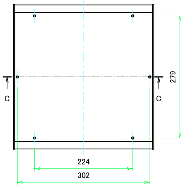
A view
