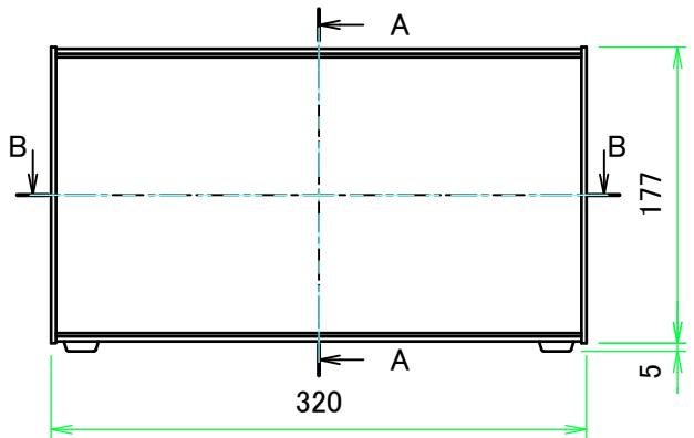
F view
