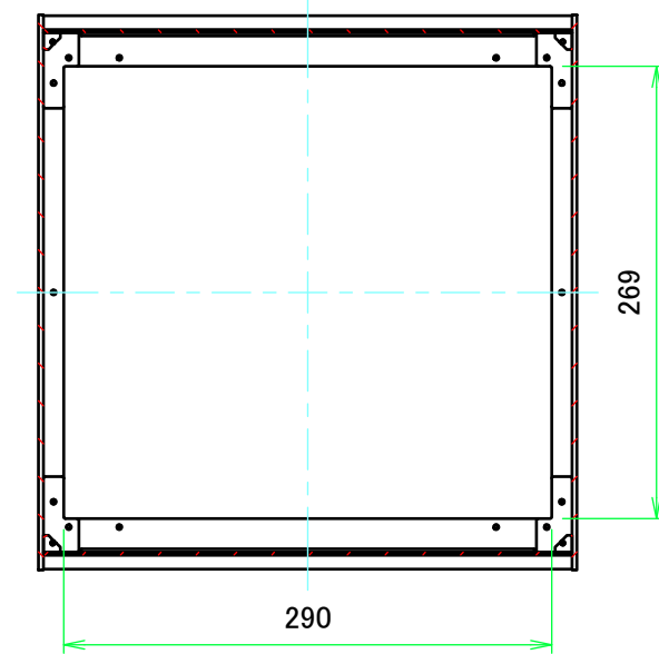
B-B (1:5)
