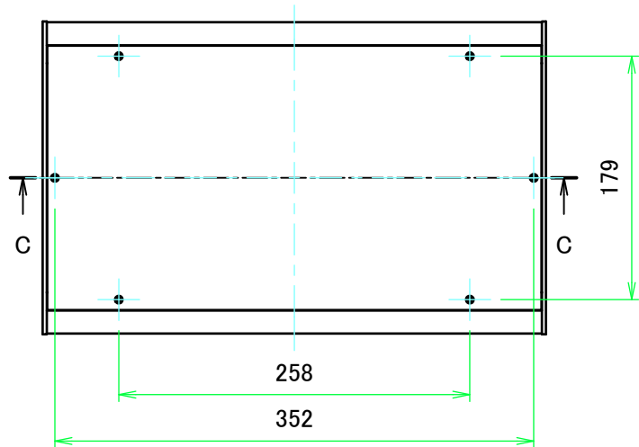
E view
