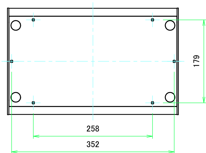
F view
