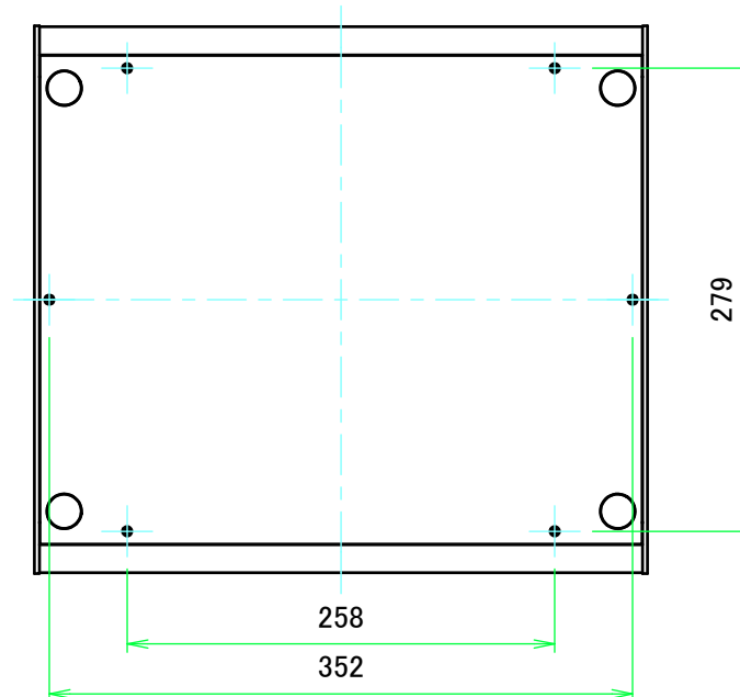
F view
