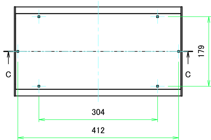
E view
