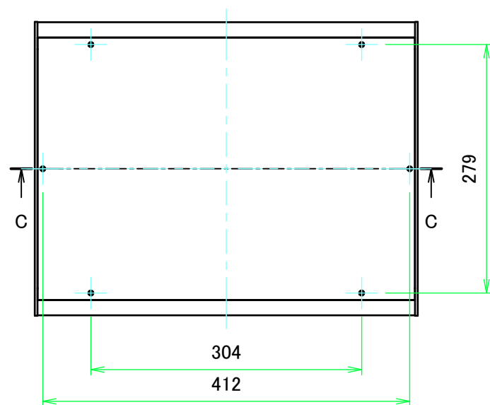
E view
