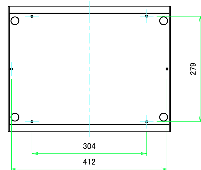
F view
