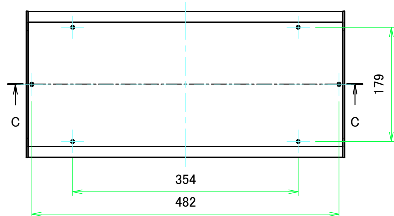
E view
