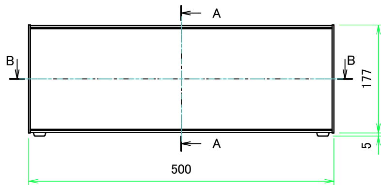
A view
