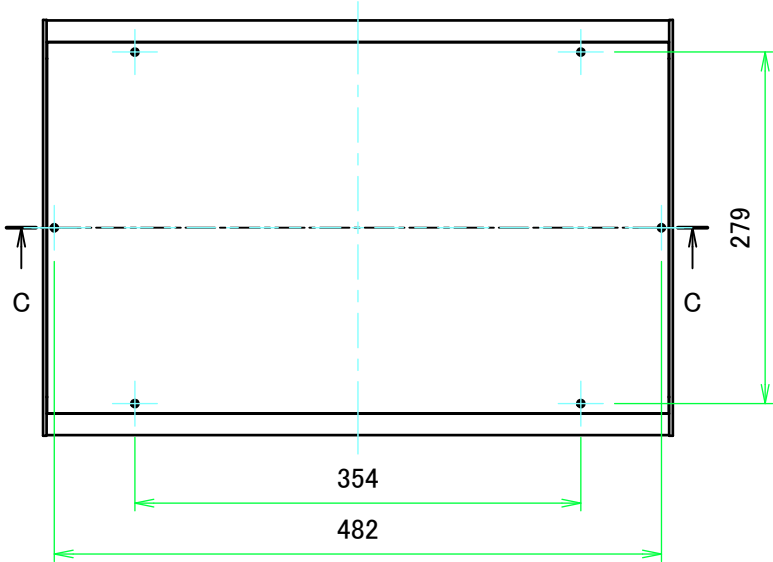
E view
