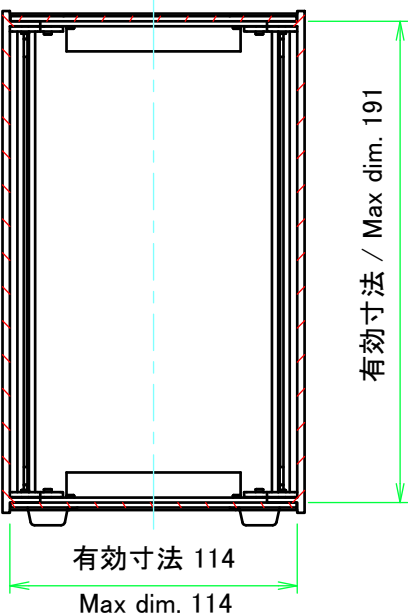
C-C (1:3)
