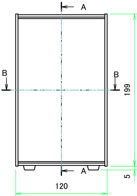
A view
