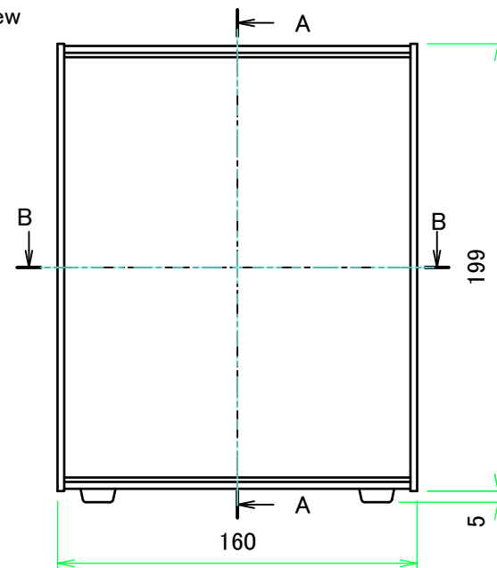
F view
