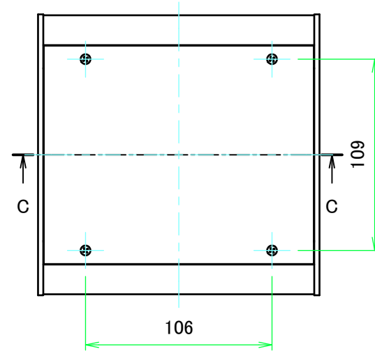
E view
