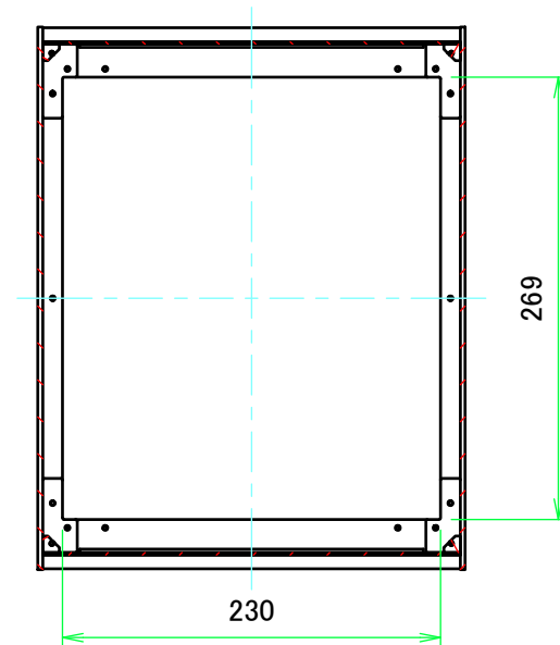
B-B (1:5)
