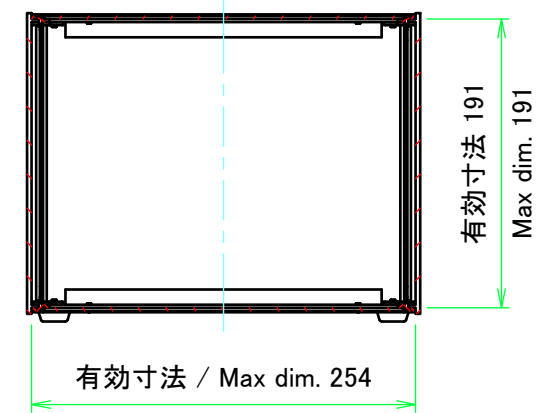
C-C (1:5)
