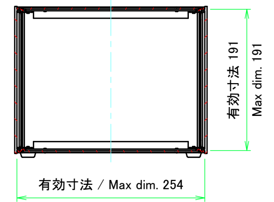
C-C (1:5)
