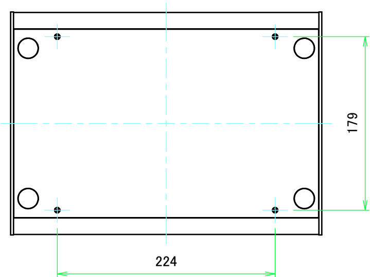
F view
