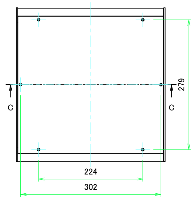
A view
