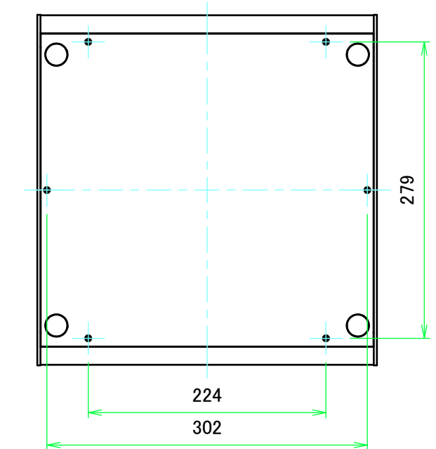
F view
