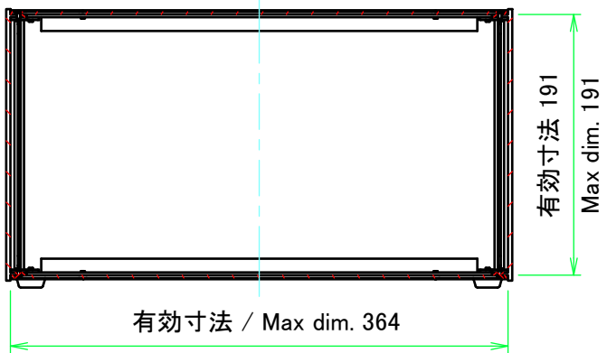
C-C (1:5)
