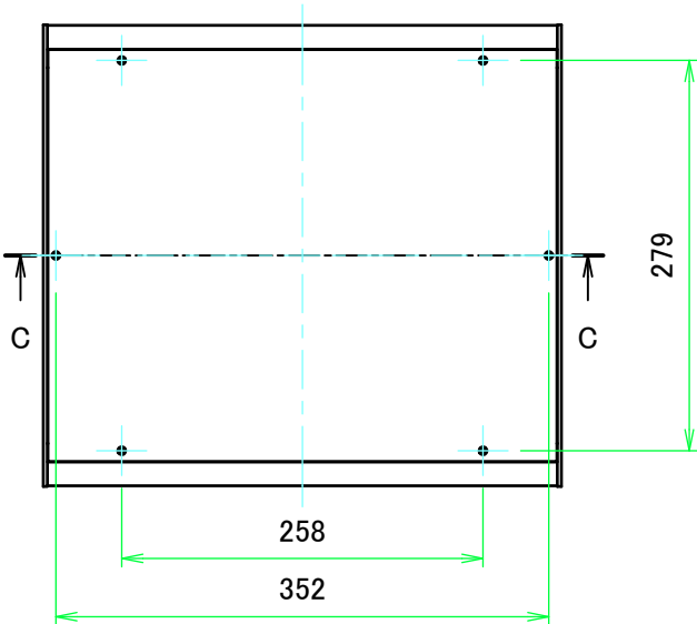
A view
