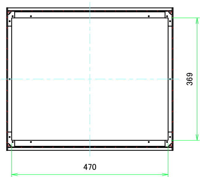
B-B (1:7)
