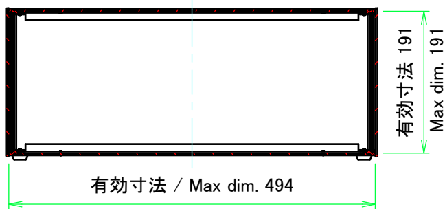
C-C (1:7)
