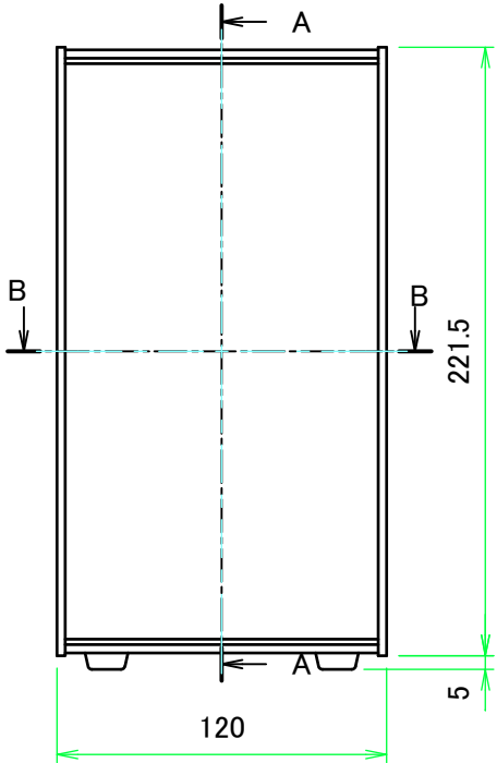
A view
