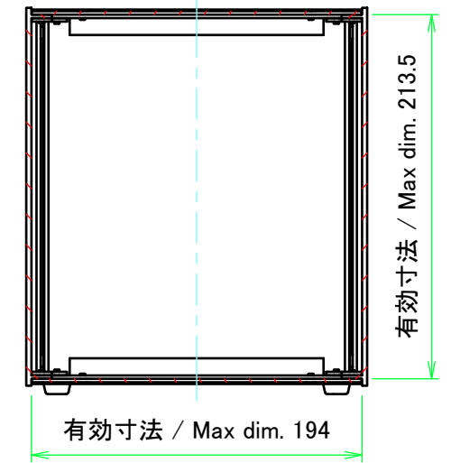
C-C (1:4)
