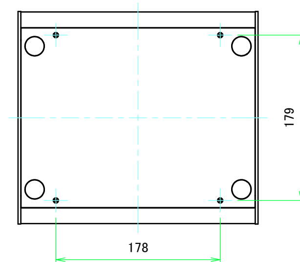
F view
