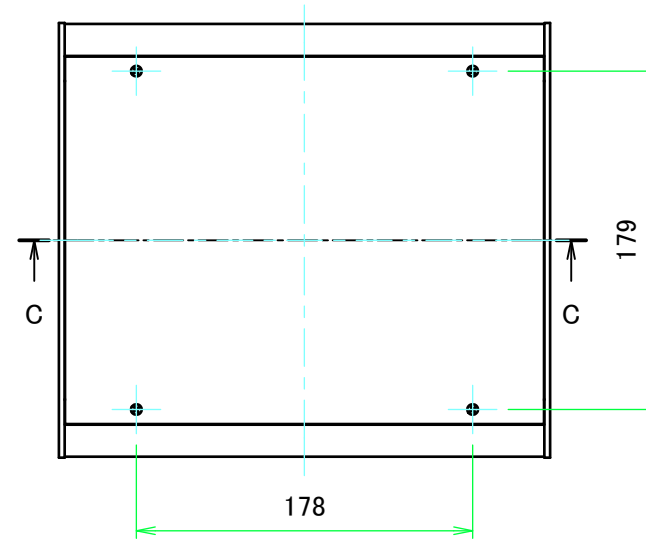
E view
