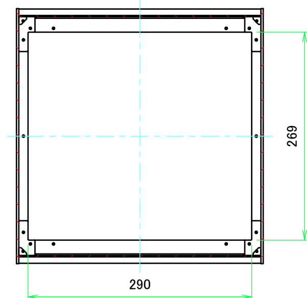
B-B (1:5)
