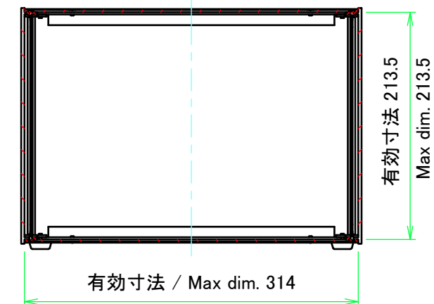
C-C (1:5)
