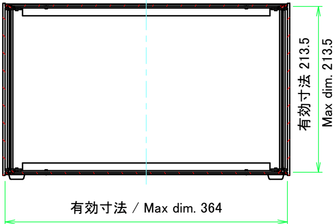
C-C (1:5)
