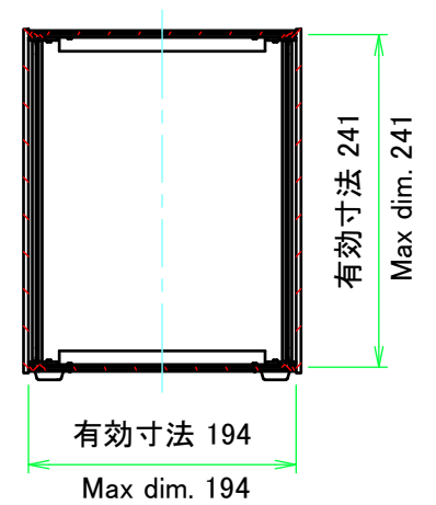
C-C (1:6)
