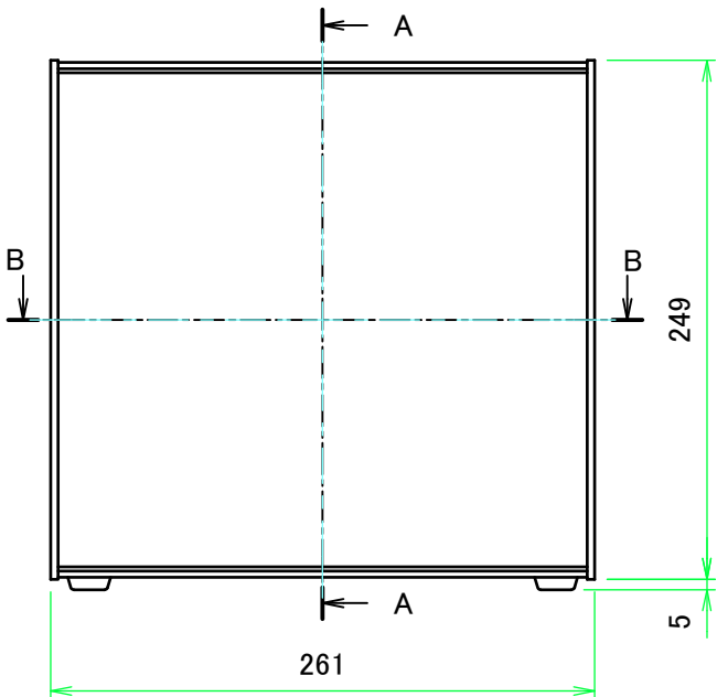
A view
