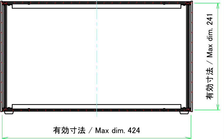
C-C (1:5)
