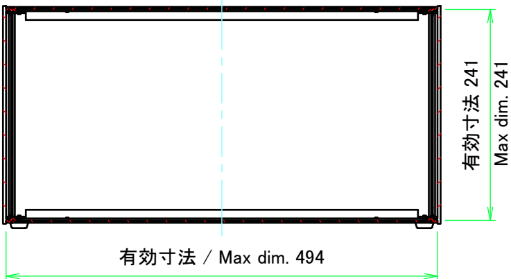
C-C (1:6)
